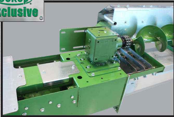
CENTER SUMP WITH OPENINGS ON BOTH SIDES OF THE GEARBOX
